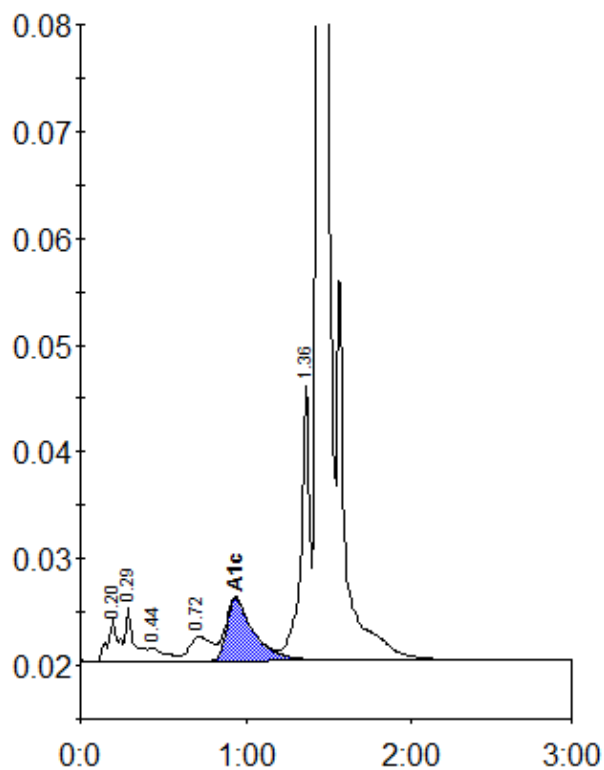
Peak table - ID: 10560464
